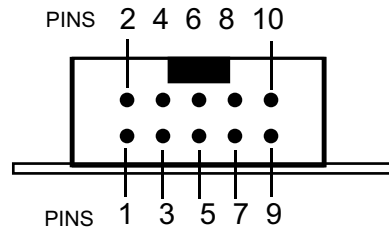
HEADER PIN-OUT FOR AR-16, EX-16 & EX-32.
